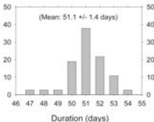
Figure 2. Distribution of incubation durations for 37 nests monitored daily during the 2013 breeding season.
