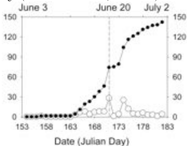
Figure 1. Number of new (white circles) and total (black circles) nests documented daily during the 2013 breeding season, showing the median egg laying date (vertical hatched line). June 3 and July 2 correspond to the first data point and right vertical axis, respectively.
