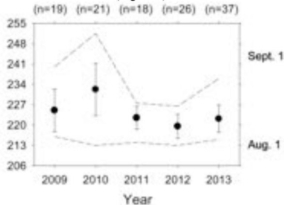
Figure 3. Comparison of hatching dates by year, showing the mean +/- SD (circles and error bars) and the range of values (hatched lines). Overall hatching dates of individual birds ranges from August 1 in 2010 / July 31 in 2012 (Julian Day 213) to September 8 (Julian Day 251) in 2010. In 2013, August 1 corresponds to Julian Day 213, while September 1 corresponds to Julian Day 244.
